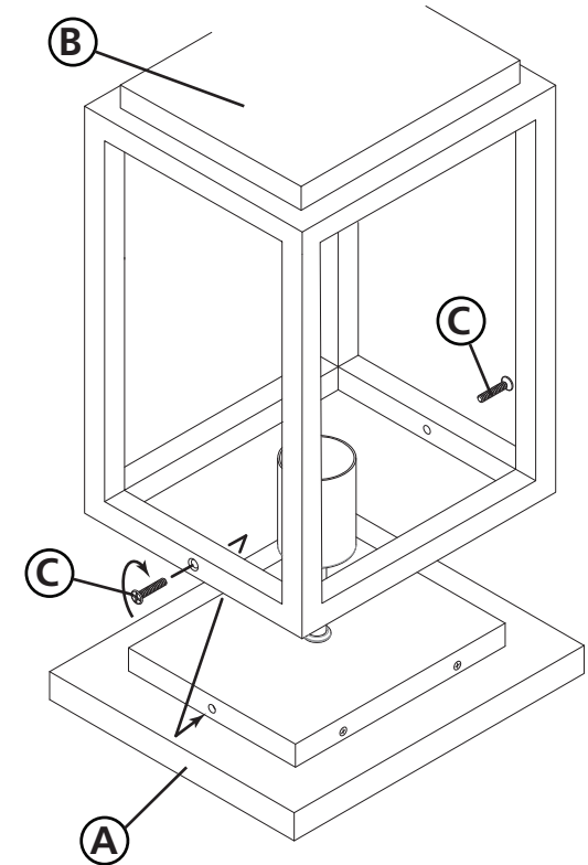
DRAWING 1 - MOUNTING
