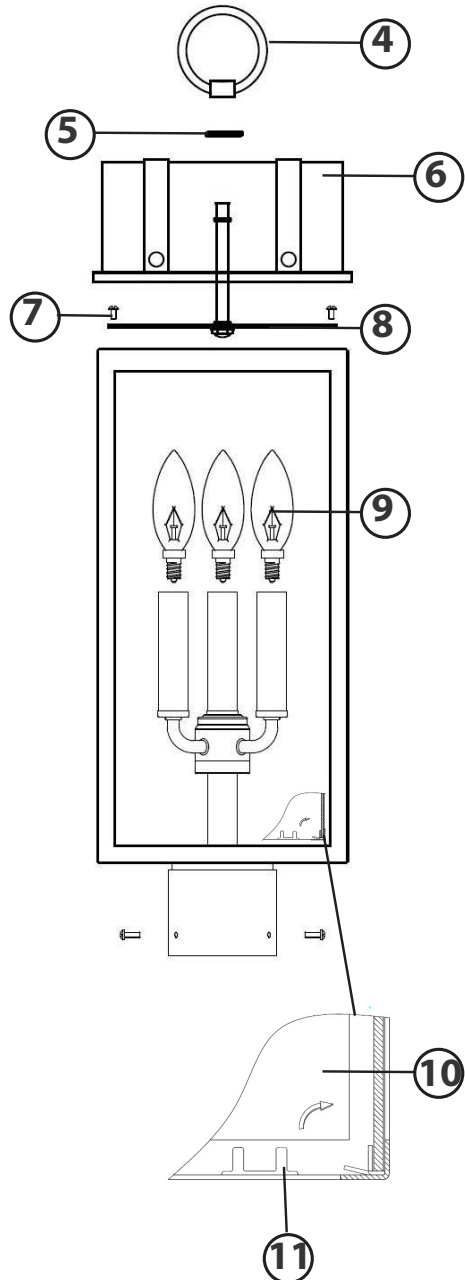
Drawing 2 - CAGE ASSEMBLY
