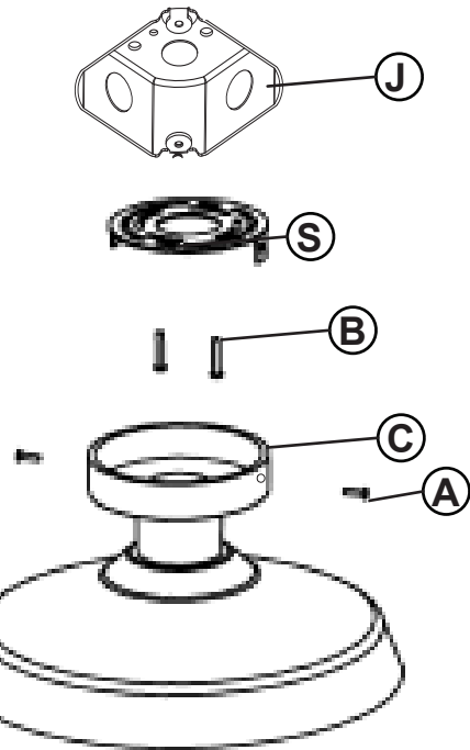
DRAWING 1 - MOUNTING
