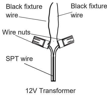
DRAWING 2- Multiple fixture wiring
