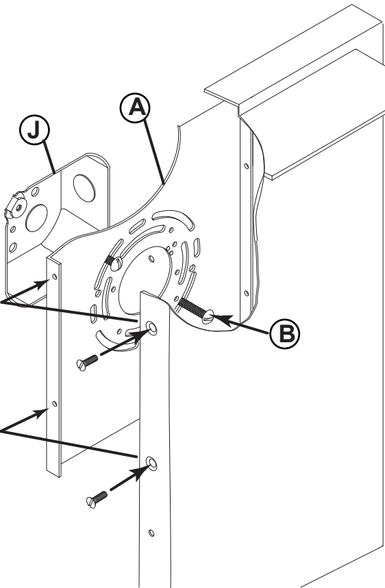
DRAWING 2 - MOUNTING
