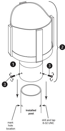
Drawing 2 – GLASS INSTALL
