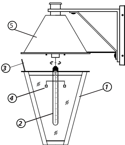
DRAWING 2-Cage Installation
