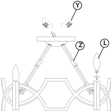
DRAWING 2- Assembly
