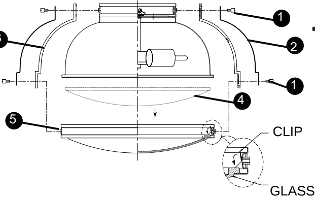
DRAWING 2 - GLASS INSTALLATION
