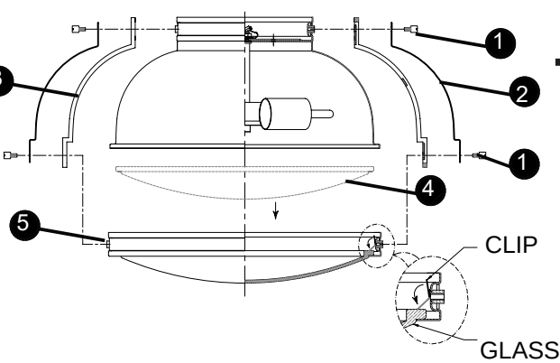
DRAWING 2 - GLASS INSTALLATION
