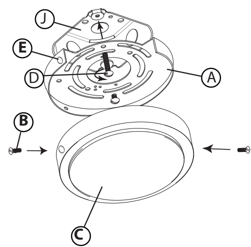
DRAWING 2- Assembly
