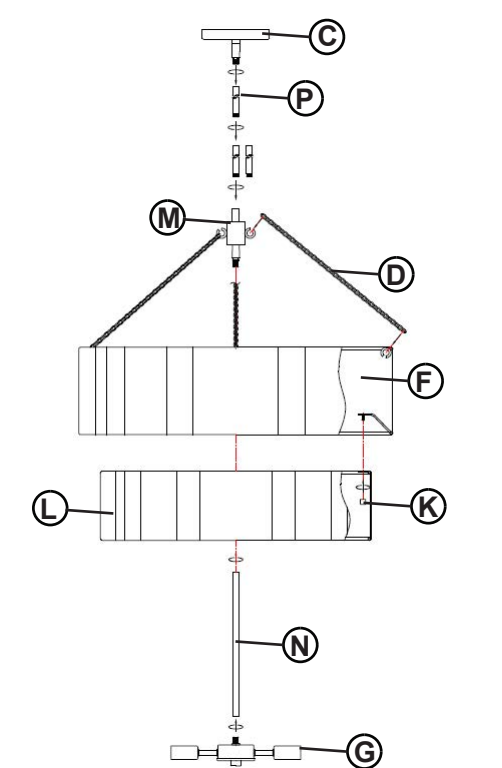
DRAWING 2- Assembly
