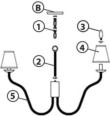
Drawing 1 – Assembly
