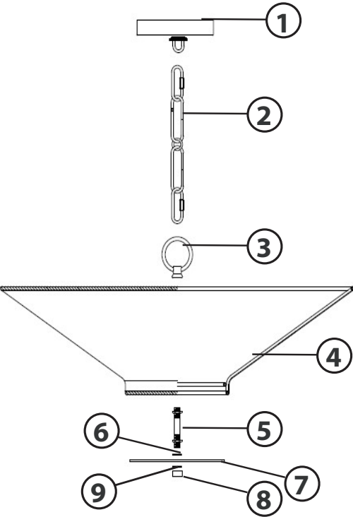
Drawing 1 - ASSEMBLY
