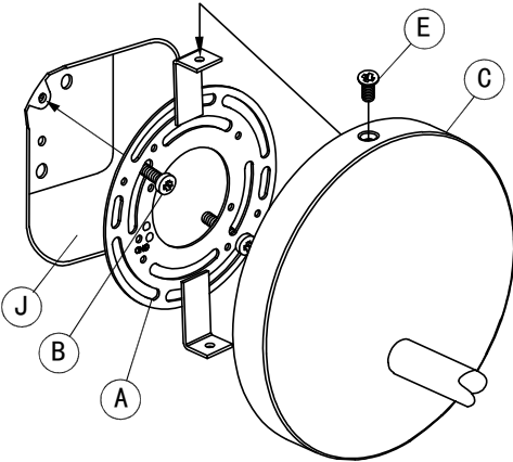
DRAWING 2- Fixture Adjustment
