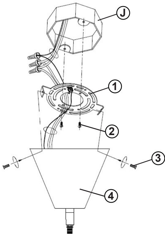
DRAWING 2 - Fixture assembly
