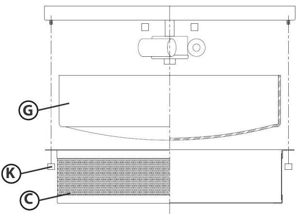
DRAWING 2 - GLASS INSTALLATION
