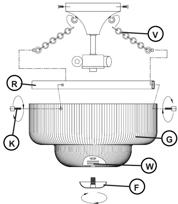
DRAWING 2- Assembly
