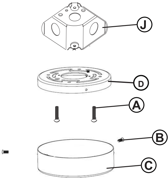
DRAWING 1 - MOUNTING
