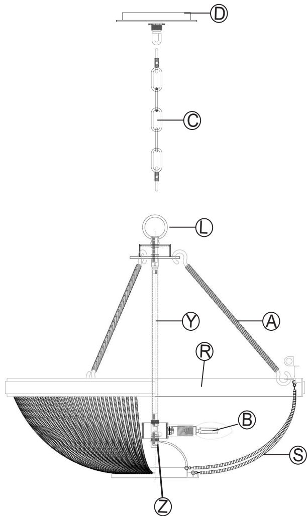
DRAWING 1 - ASSEMBLY
