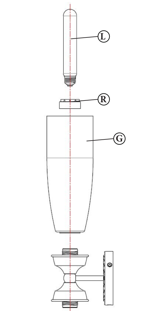
DRAWING 2-
