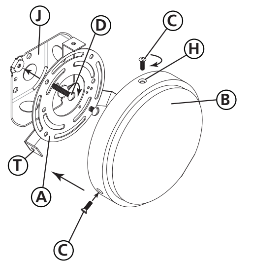
DRAWING 2-
