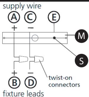
Drawing 2 – Chain Hanging
