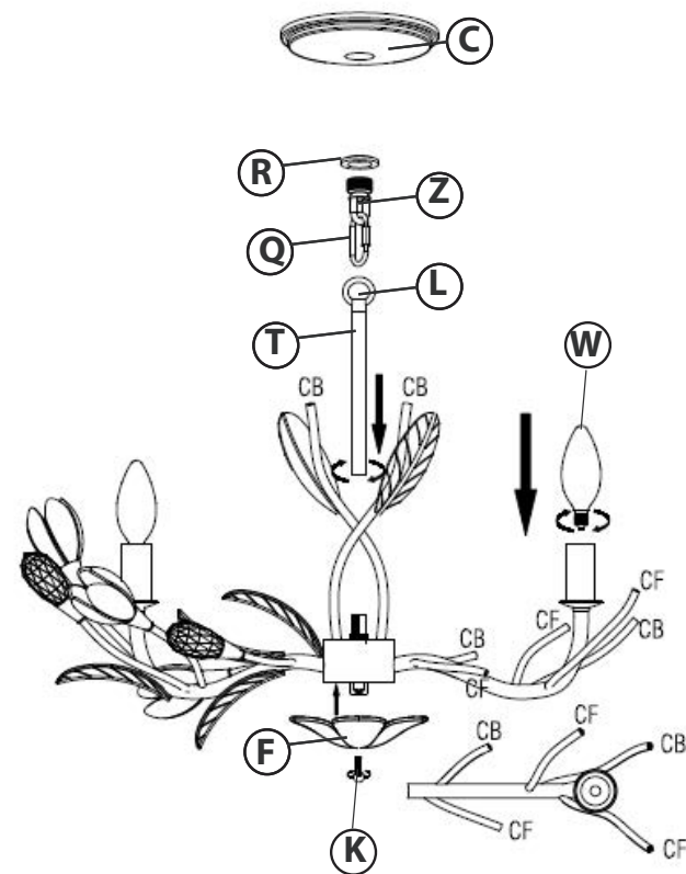
DRAWING 1 - Fixture Installation
