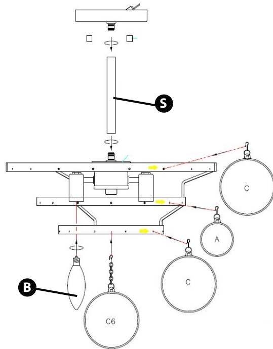
DRAWING 2 - Assembly
