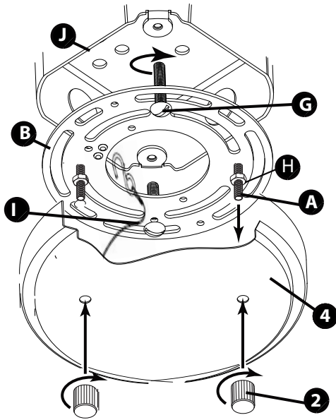
DRAWING 2 - Assembly
