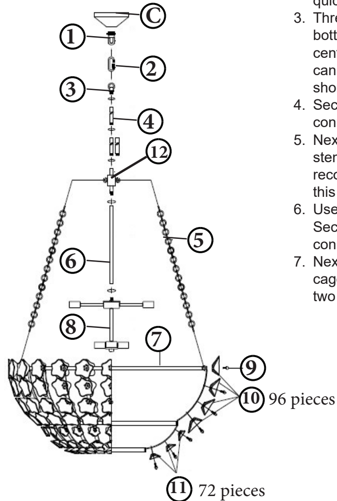
DRAWING 1 - Assembly
