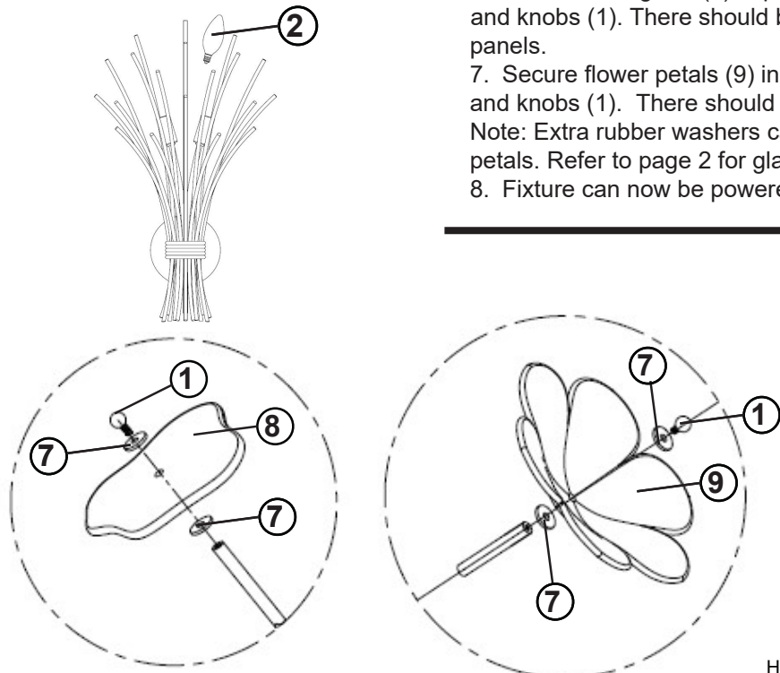
DRAWING 2 -Petal assembly
