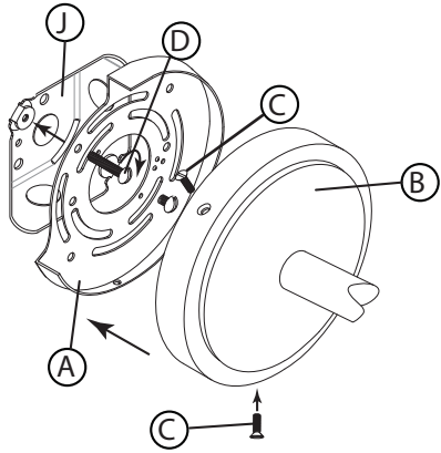
DRAWING 1 - MOUNTING
