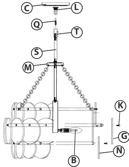
Drawing 1- Assembly
