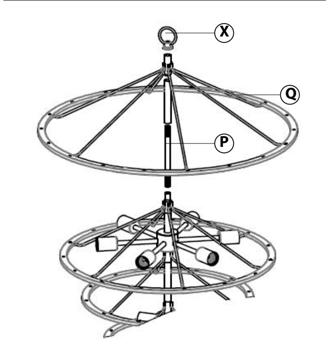
DRAWING 2 - Assembly
