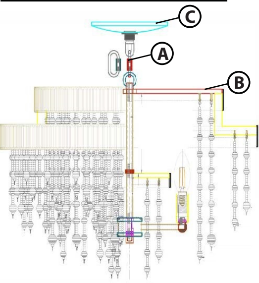
Drawing 1- Assembly
